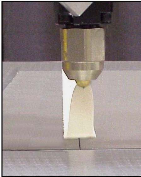
1208-206-.020 Slot Nozzle Applying PVC Seam Sealer
