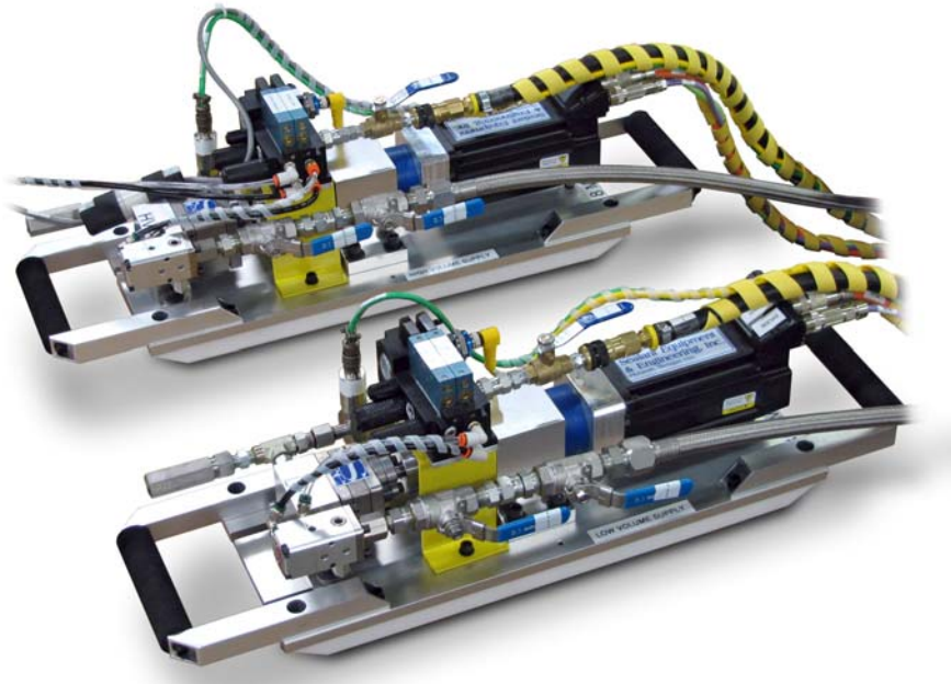
Servo-Flo 704-PGM Portable Gear Meter
