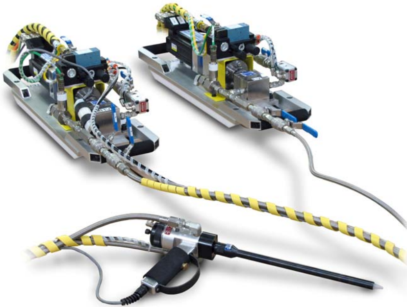
Servo-Flo 704-PGM Portable Gear Meter System Mounted on Individual No-Mar Skid Plates
